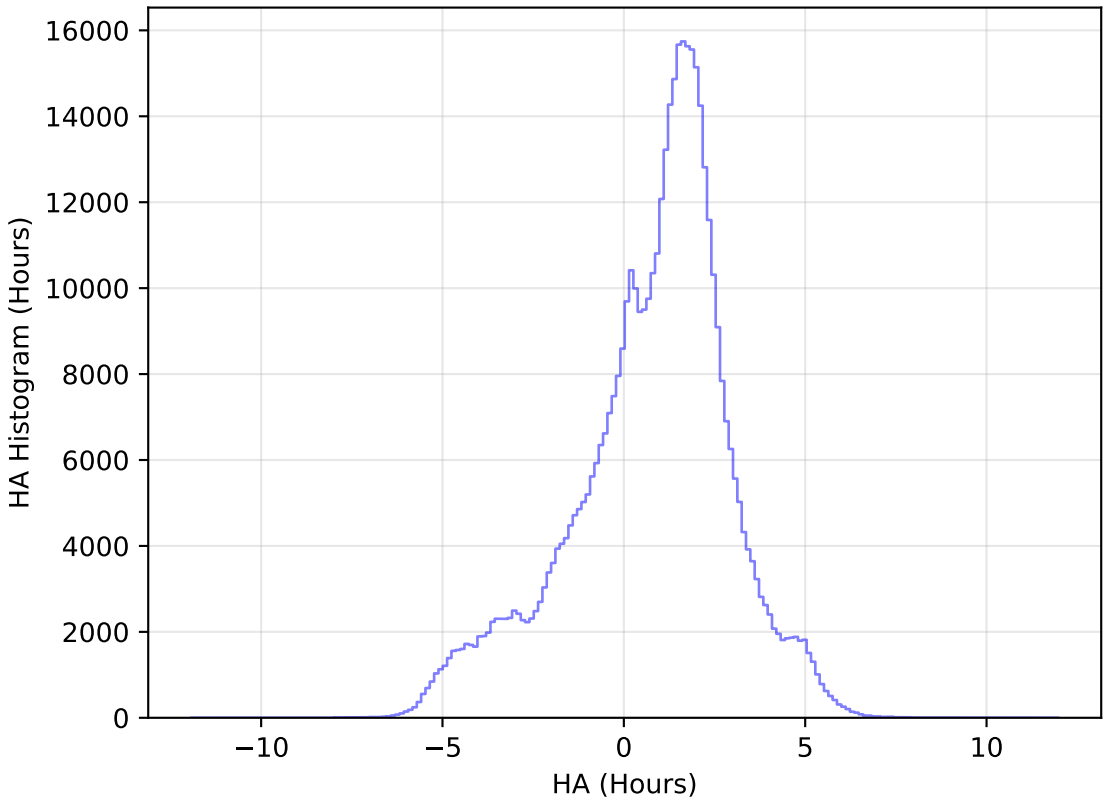
too_elab_r64_d2_gz_v3.4_10yrs All sky i band: HA Histogram
