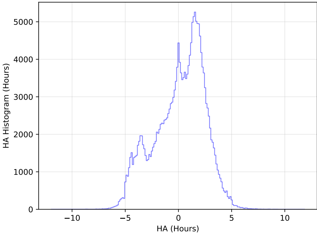
too_elab_r64_d2_gz_v3.4_10yrs All sky g band: HA Histogram
