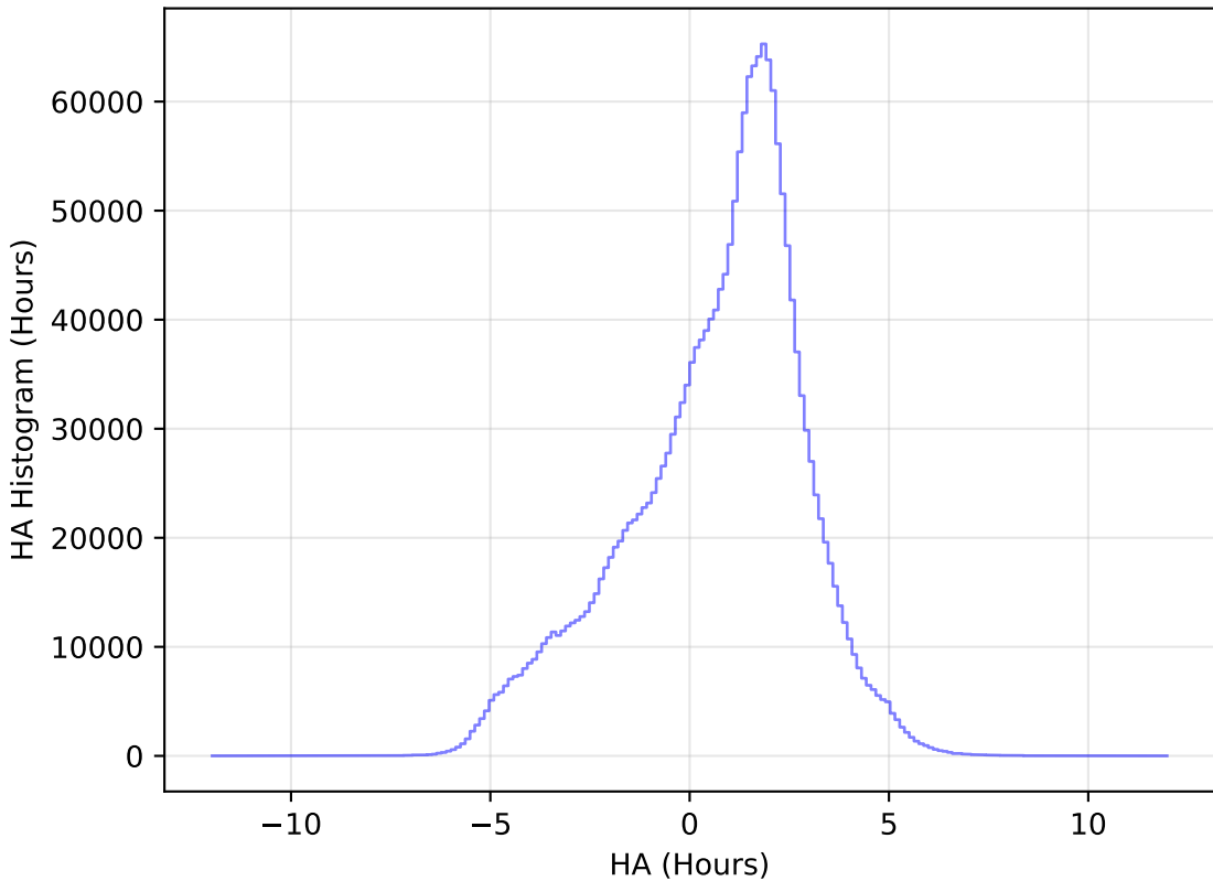
too_elab_r64_d2_gz_v3.4_10yrs All sky all bands: HA Histogram
