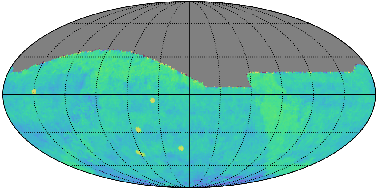
too_elab_r64_d2_gz_v3.4_10yrs gri All sky: Fraction of visits in pairs (10-60 min)
