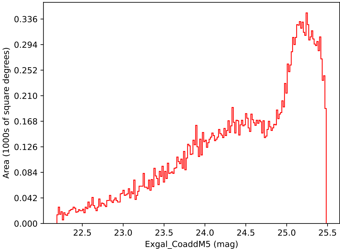
too_elab_r64_d2_gz_v3.4_10yrs Yr 3-4 i band: Exgal_CoaddM5
