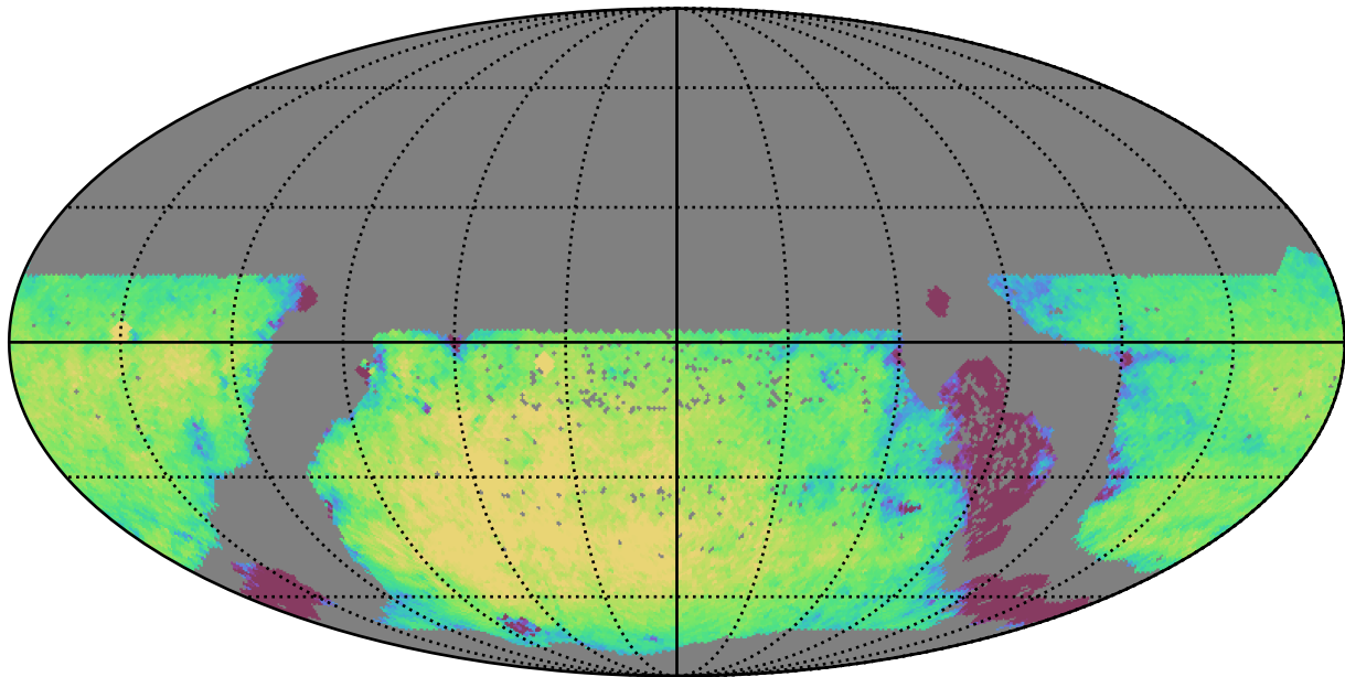
too_elab_r64_d2_gz_v3.4_10yrs WFD g band: Exgal_CoaddM5
