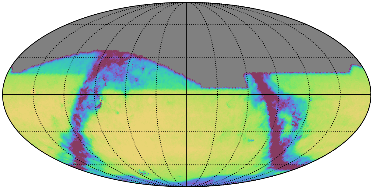
too_elab_r64_d2_gz_v3.4_10yrs All sky i band: Exgal_CoaddM5
