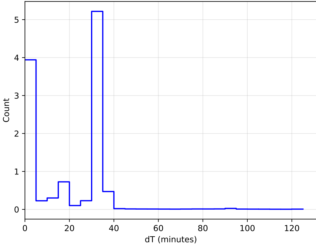
too_elab_r64_d2_gz_v3.4_10yrs WFD: DeltaT Histogram
