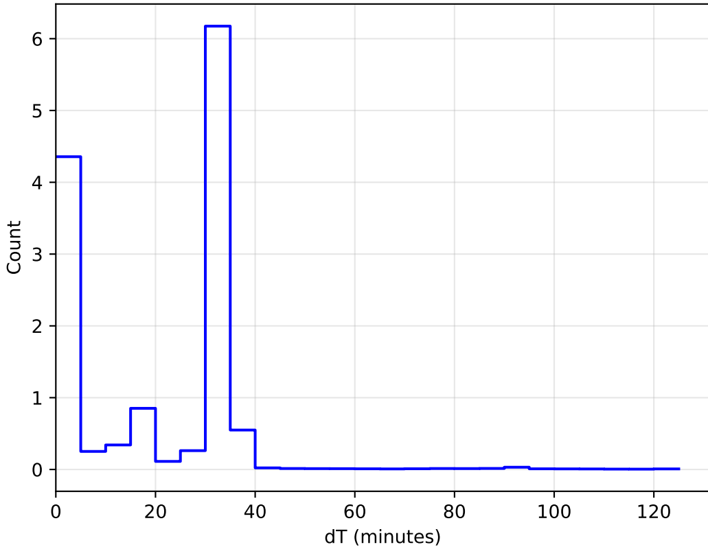
too_elab_r64_d2_gz_v3.4_10yrs All sky: DeltaT Histogram 1e6
