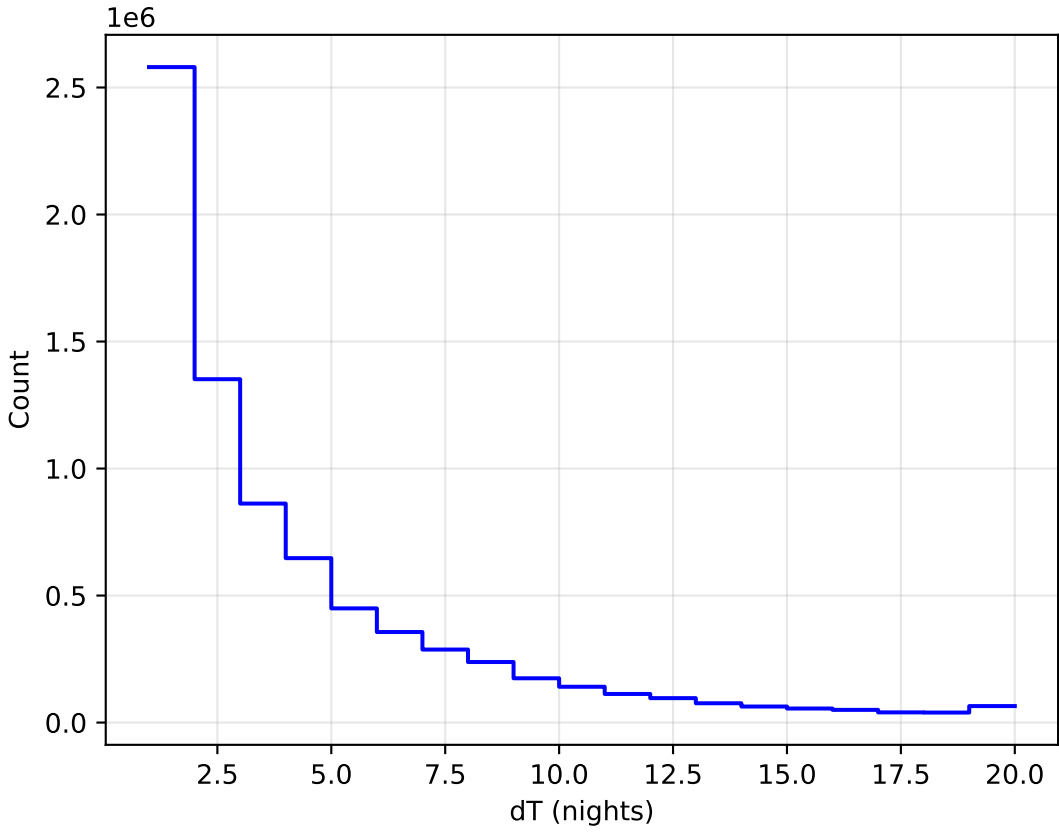
too_elab_r64_d2_gz_v3.4_10yrs WFD all bands: DeltaNight Histogram
