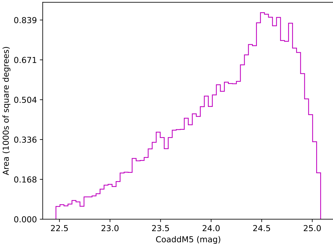
too_elab_r64_d2_gz_v3.4_10yrs Yr 3-4 z band: CoaddM5
