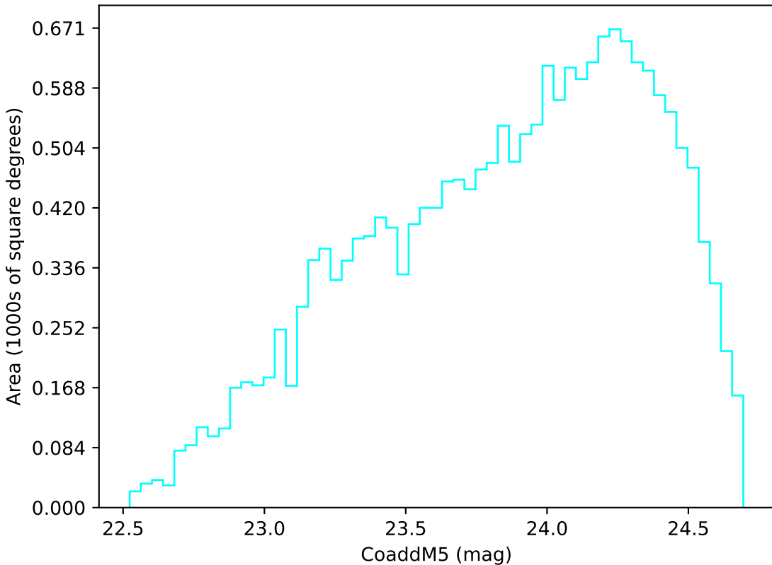
too_elab_r64_d2_gz_v3.4_10yrs Yr 3-4 u band: CoaddM5
