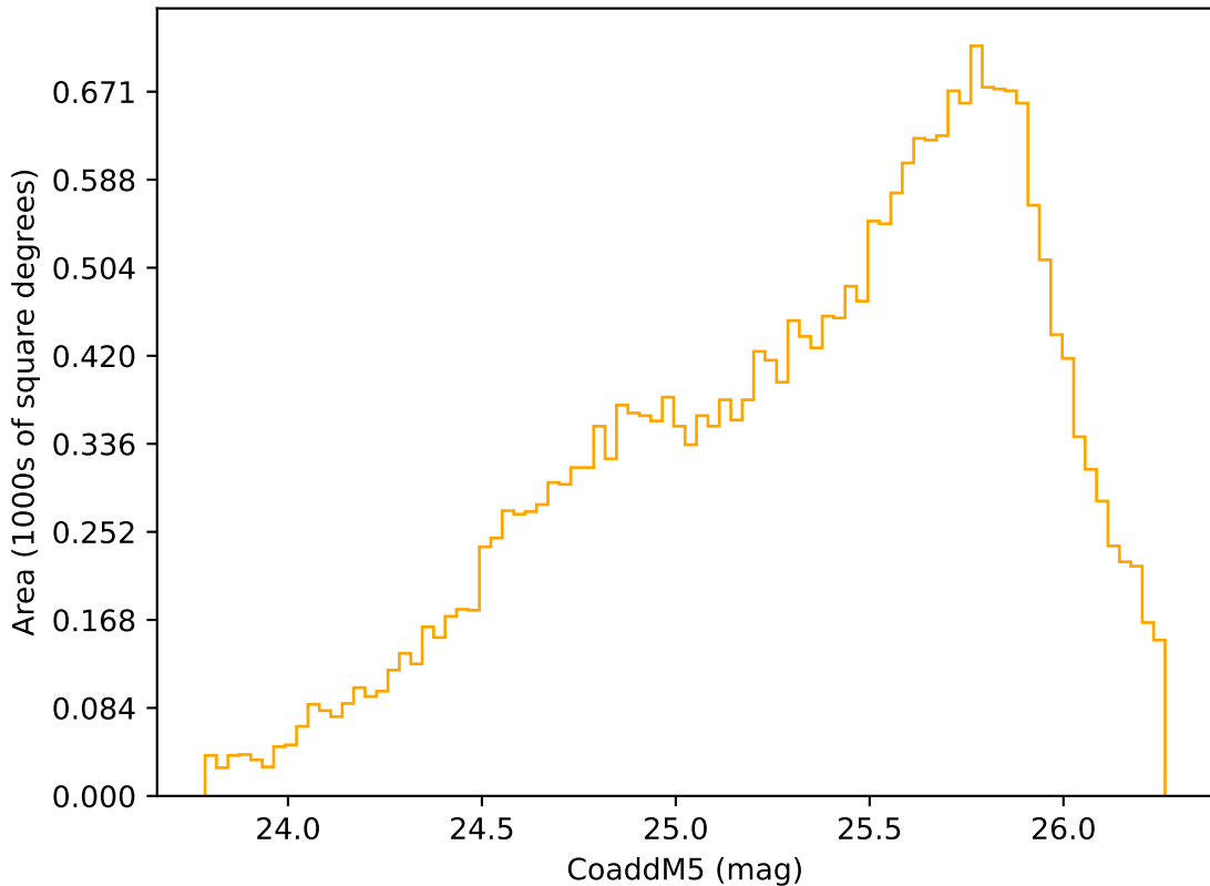
too_elab_r64_d2_gz_v3.4_10yrs Yr 3-4 r band: CoaddM5
