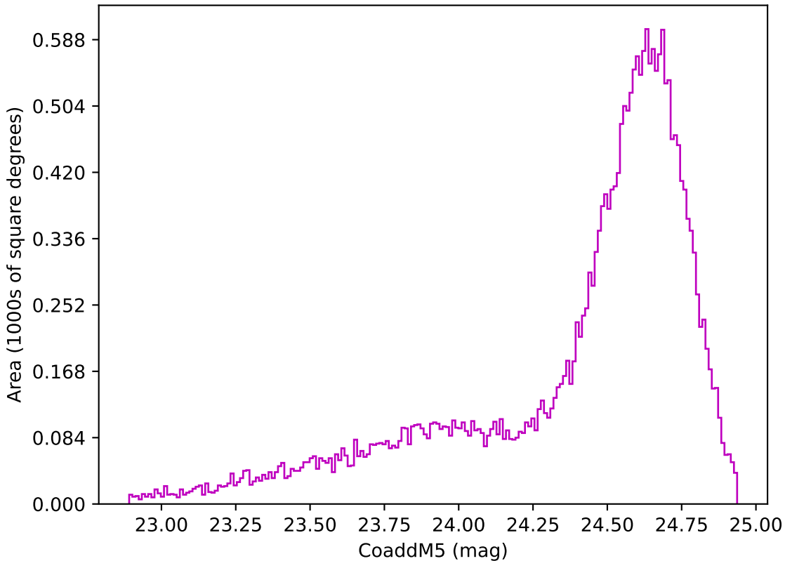
too_elab_r64_d2_gz_v3.4_10yrs Yr 1 z band: CoaddM5
