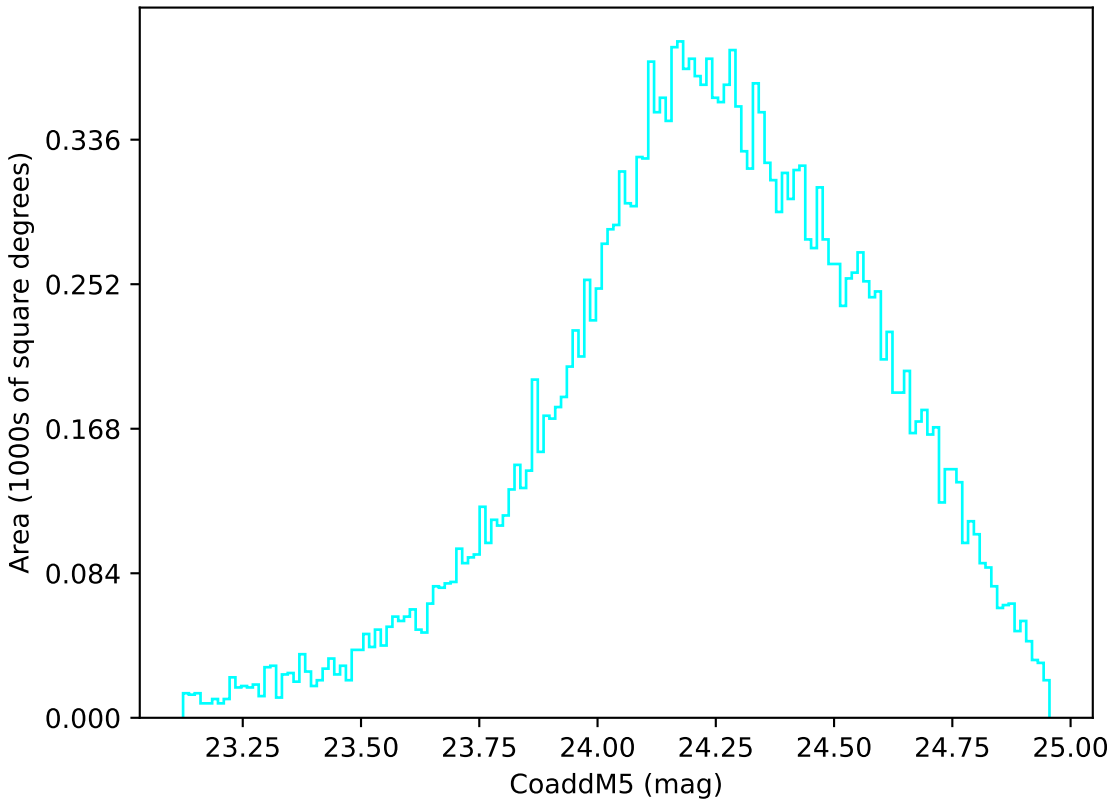
too_elab_r64_d2_gz_v3.4_10yrs Yr 1 u band: CoaddM5
