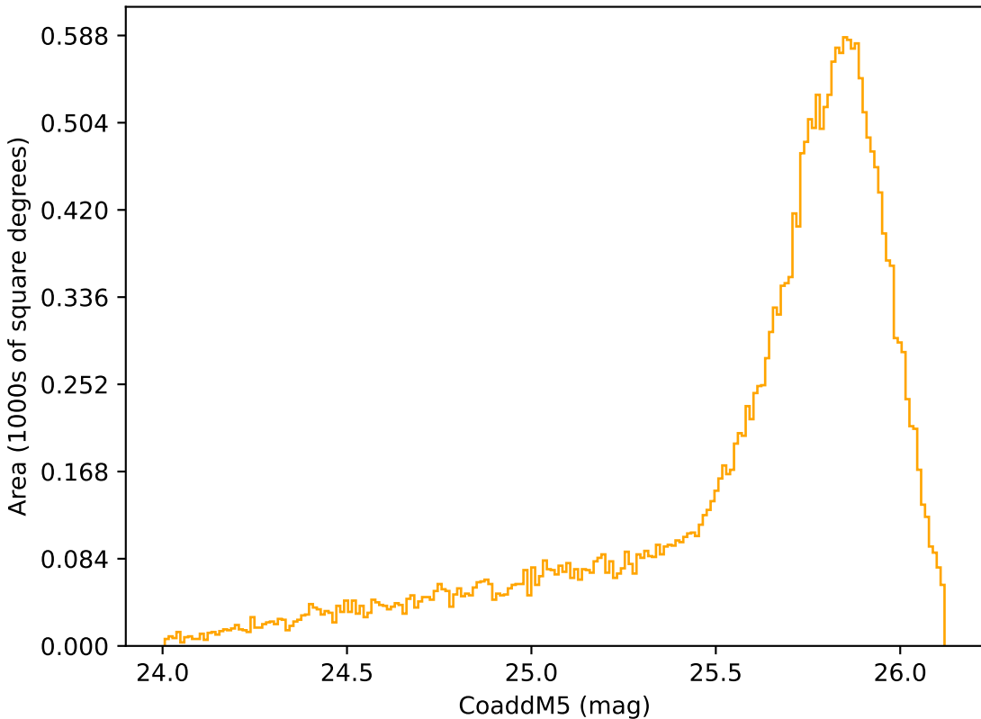
too_elab_r64_d2_gz_v3.4_10yrs Yr 1 r band: CoaddM5
