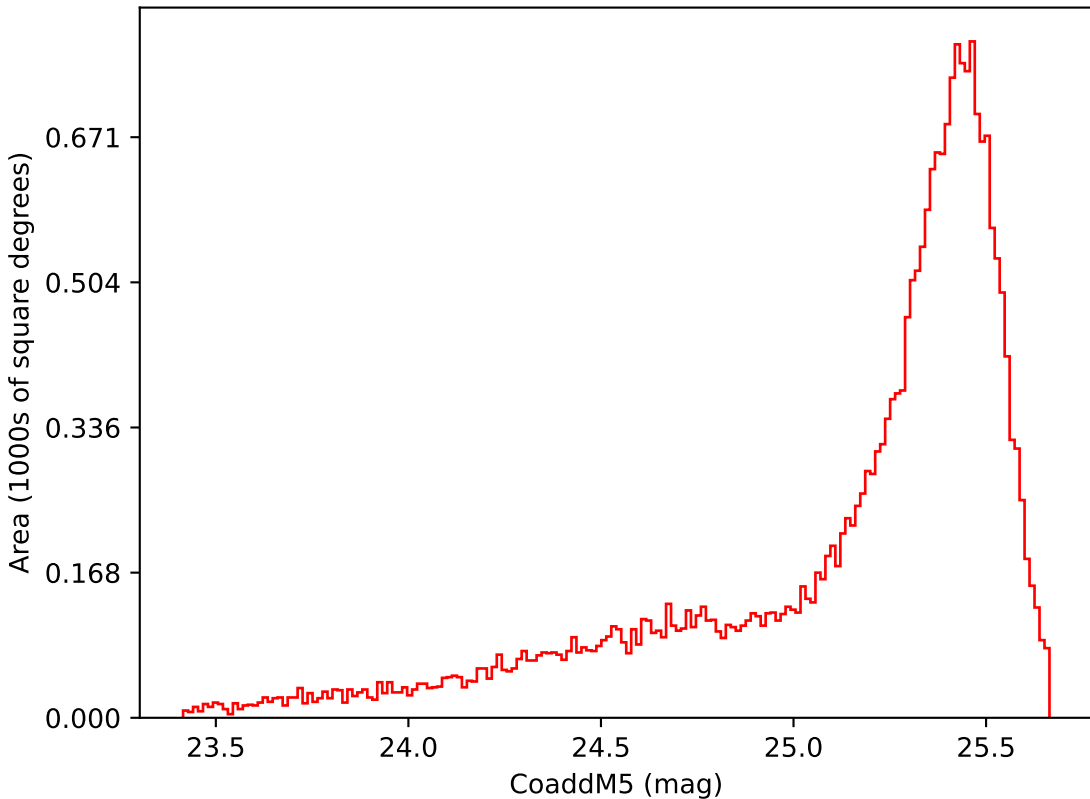
too_elab_r64_d2_gz_v3.4_10yrs Yr 1 i band: CoaddM5
