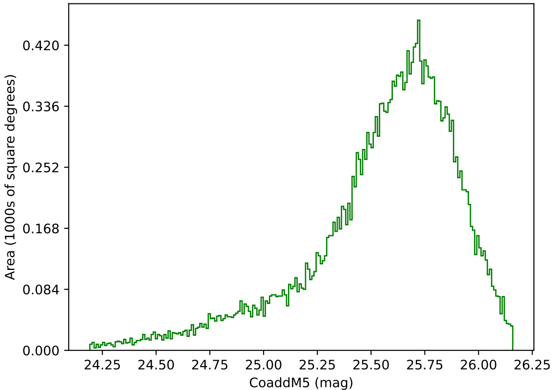
too_elab_r64_d2_gz_v3.4_10yrs Yr 1 g band: CoaddM5
