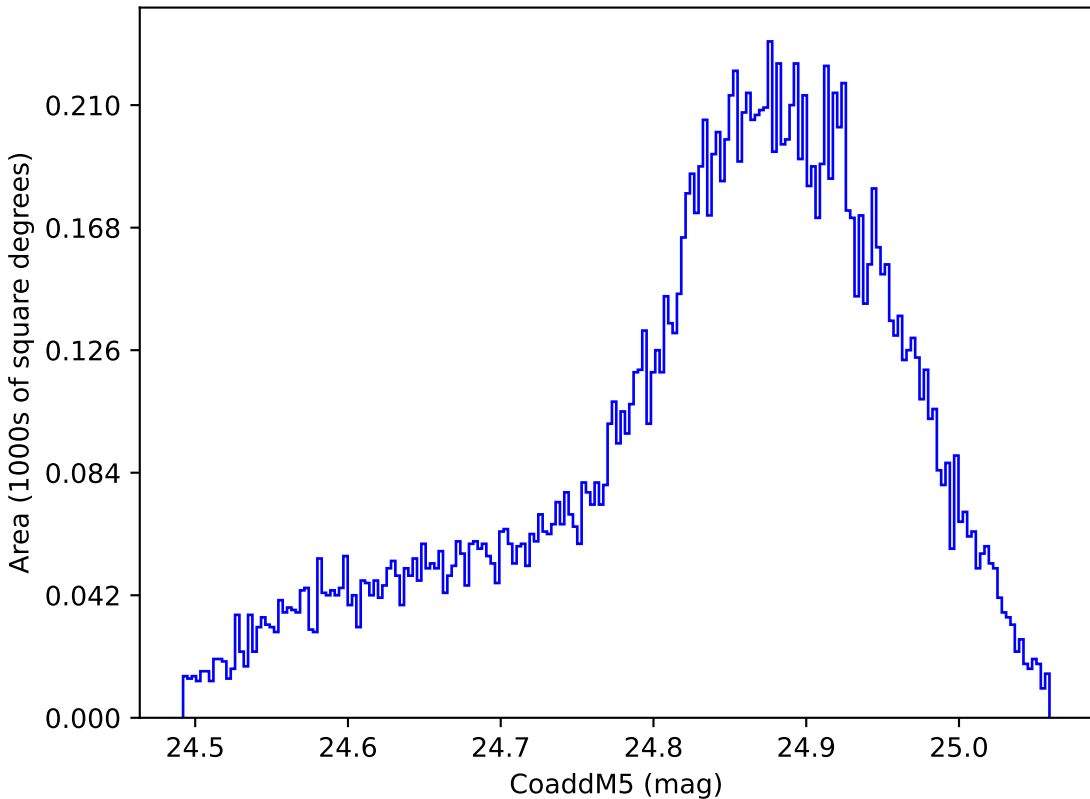
too_elab_r64_d2_gz_v3.4_10yrs WFD y band: CoaddM5
