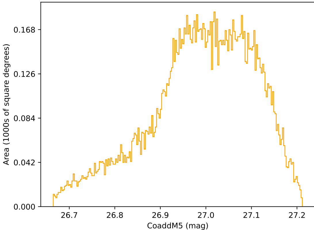
too_elab_r64_d2_gz_v3.4_10yrs WFD r band: CoaddM5
