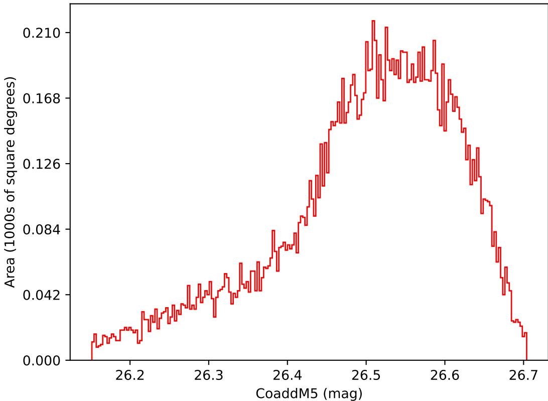
too_elab_r64_d2_gz_v3.4_10yrs WFD i band: CoaddM5
