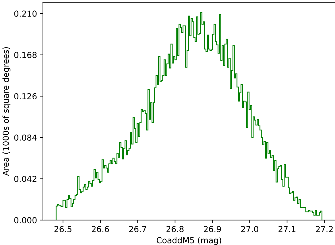
too_elab_r64_d2_gz_v3.4_10yrs WFD g band: CoaddM5
