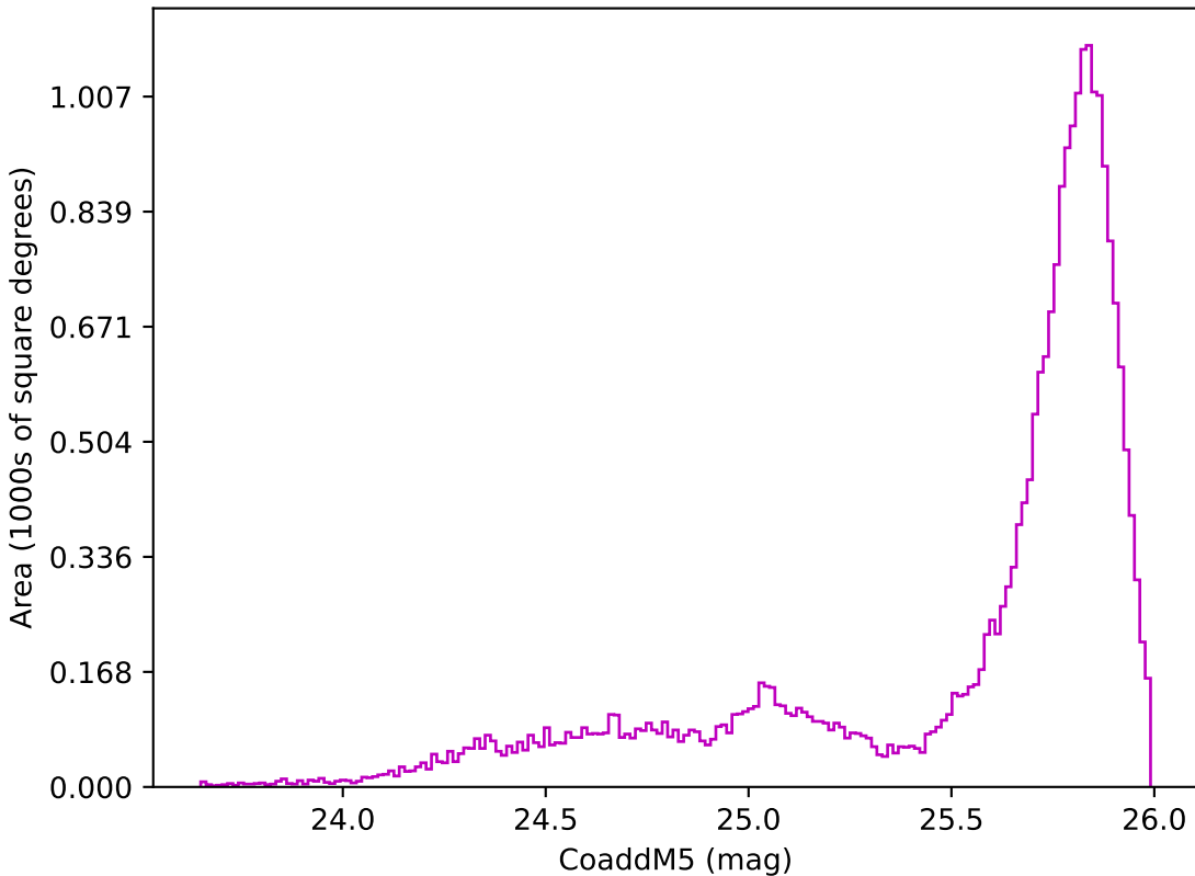
too_elab_r64_d2_gz_v3.4_10yrs All sky z band: CoaddM5
