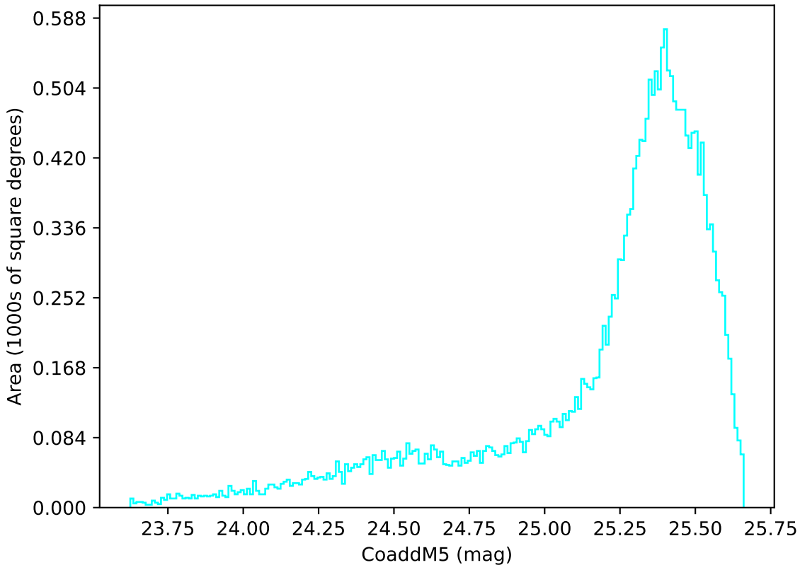
too_elab_r64_d2_gz_v3.4_10yrs All sky u band: CoaddM5
