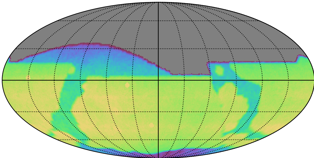
too_elab_r64_d2_gz_v3.4_10yrs All sky r band: CoaddM5
