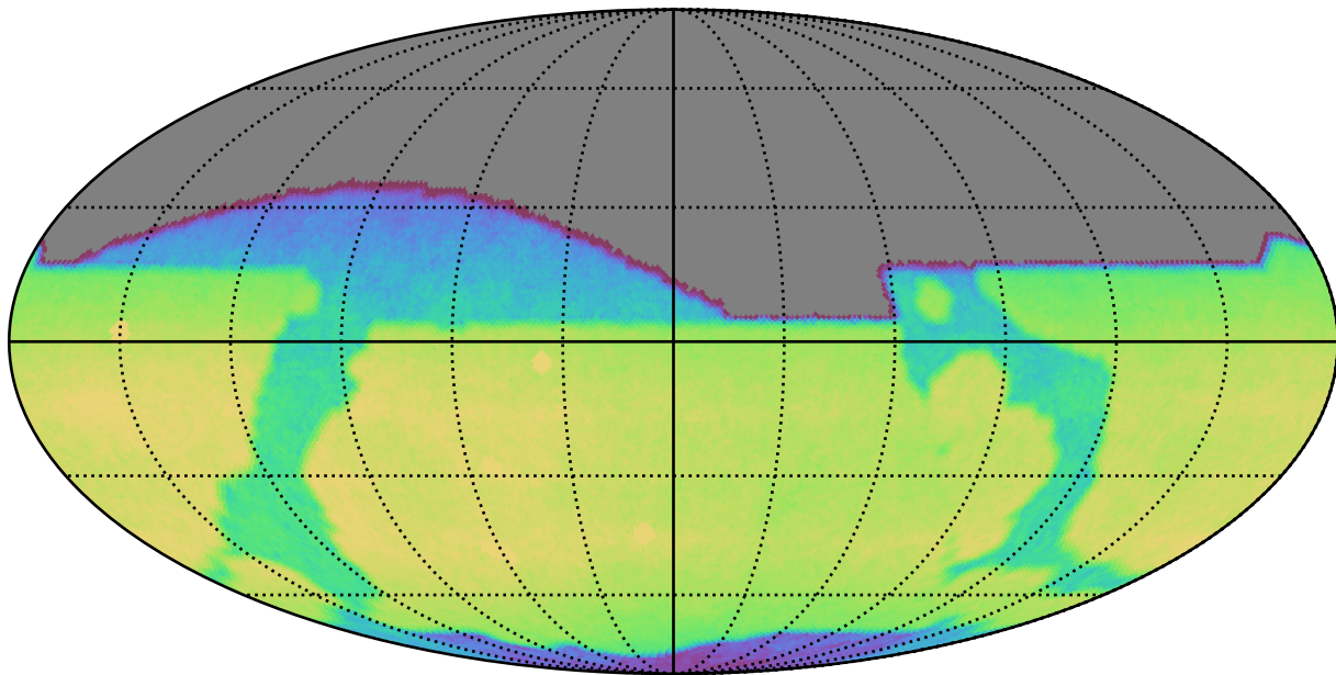
too_elab_r64_d2_gz_v3.4_10yrs All sky i band: CoaddM5
