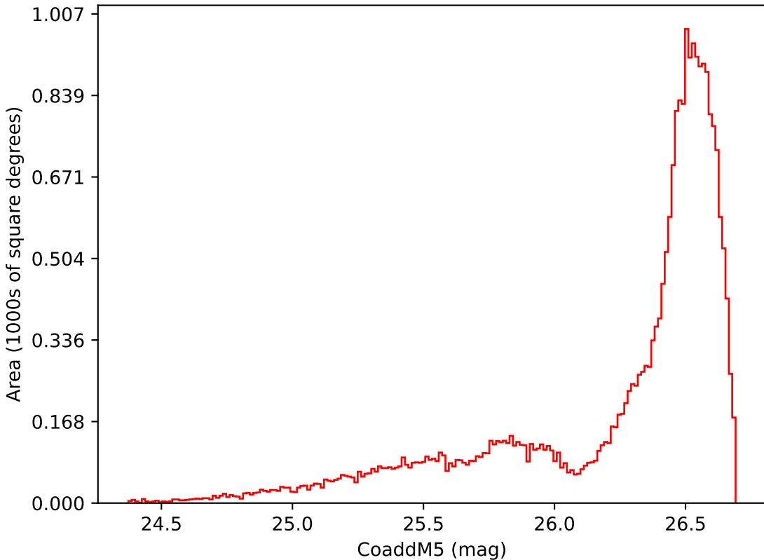
too_elab_r64_d2_gz_v3.4_10yrs All sky i band: CoaddM5
