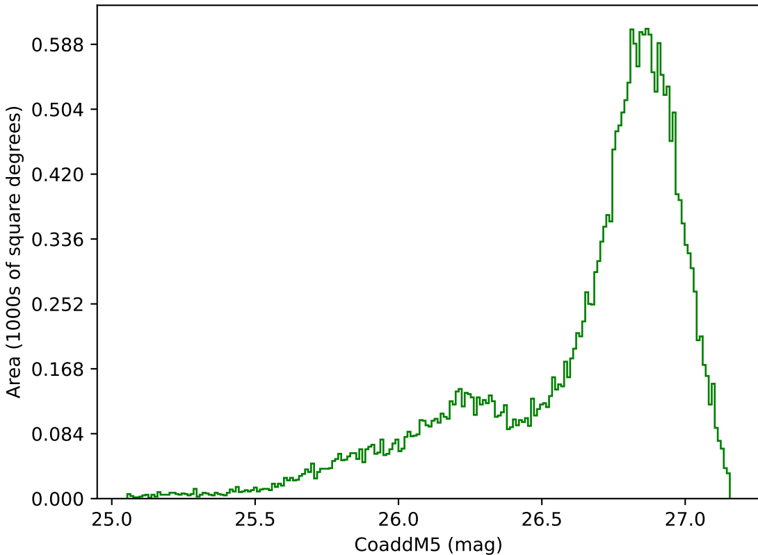
too_elab_r64_d2_gz_v3.4_10yrs All sky g band: CoaddM5
