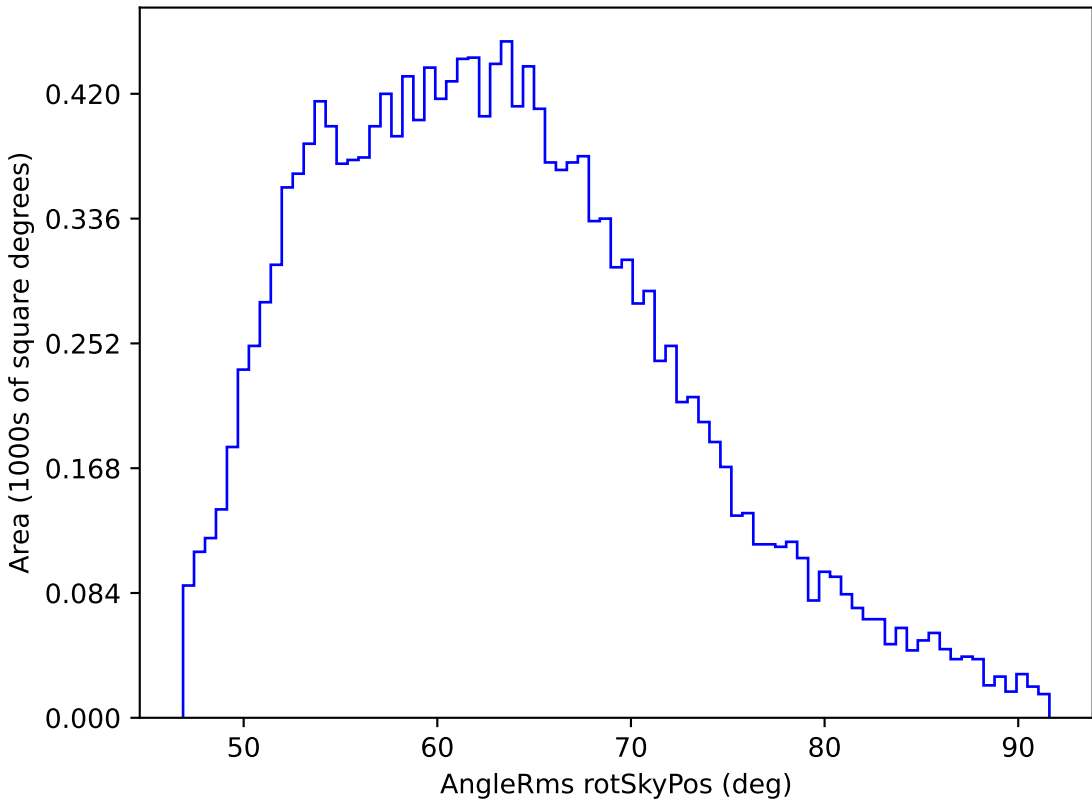
too_elab_r64_d2_gz_v3.4_10yrs WFD y band: AngleRms rotSkyPos
