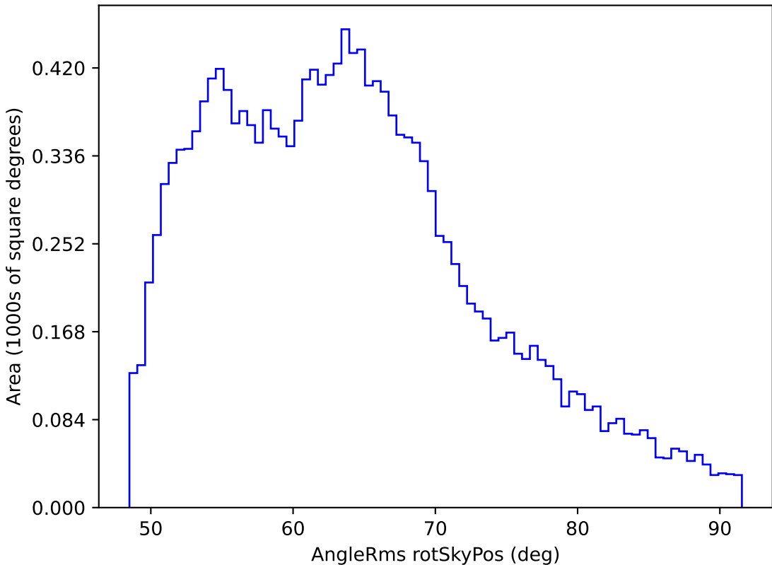
too_elab_r64_d2_gz_v3.4_10yrs WFD i band: AngleRms rotSkyPos
