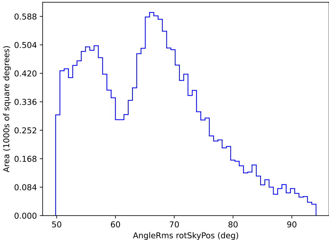
too_elab_r64_d2_gz_v3.4_10yrs WFD all bands: AngleRms rotSkyPos
