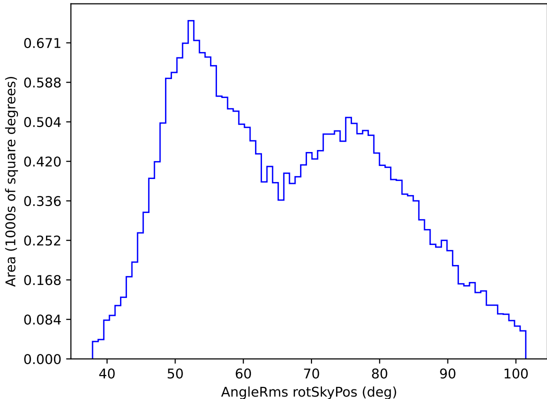
too_elab_r64_d2_gz_v3.4_10yrs All sky g band: AngleRms rotSkyPos
