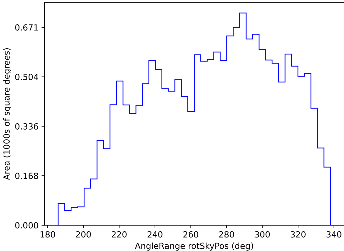
too_elab_r64_d2_gz_v3.4_10yrs WFD y band: AngleRange rotSkyPos
