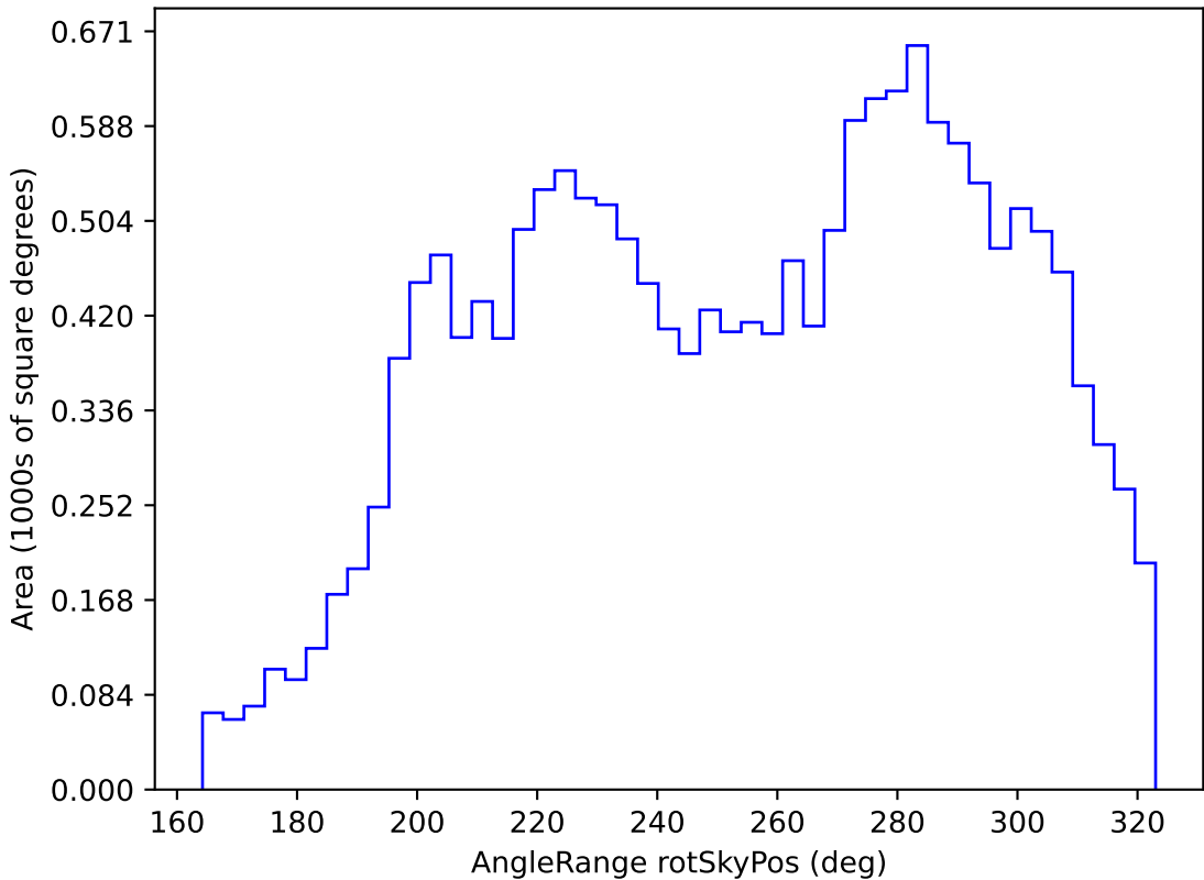
too_elab_r64_d2_gz_v3.4_10yrs WFD u band: AngleRange rotSkyPos
