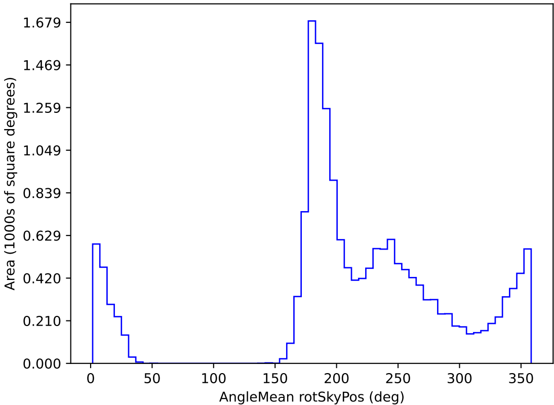
too_elab_r64_d2_gz_v3.4_10yrs WFD z band: AngleMean rotSkyPos
