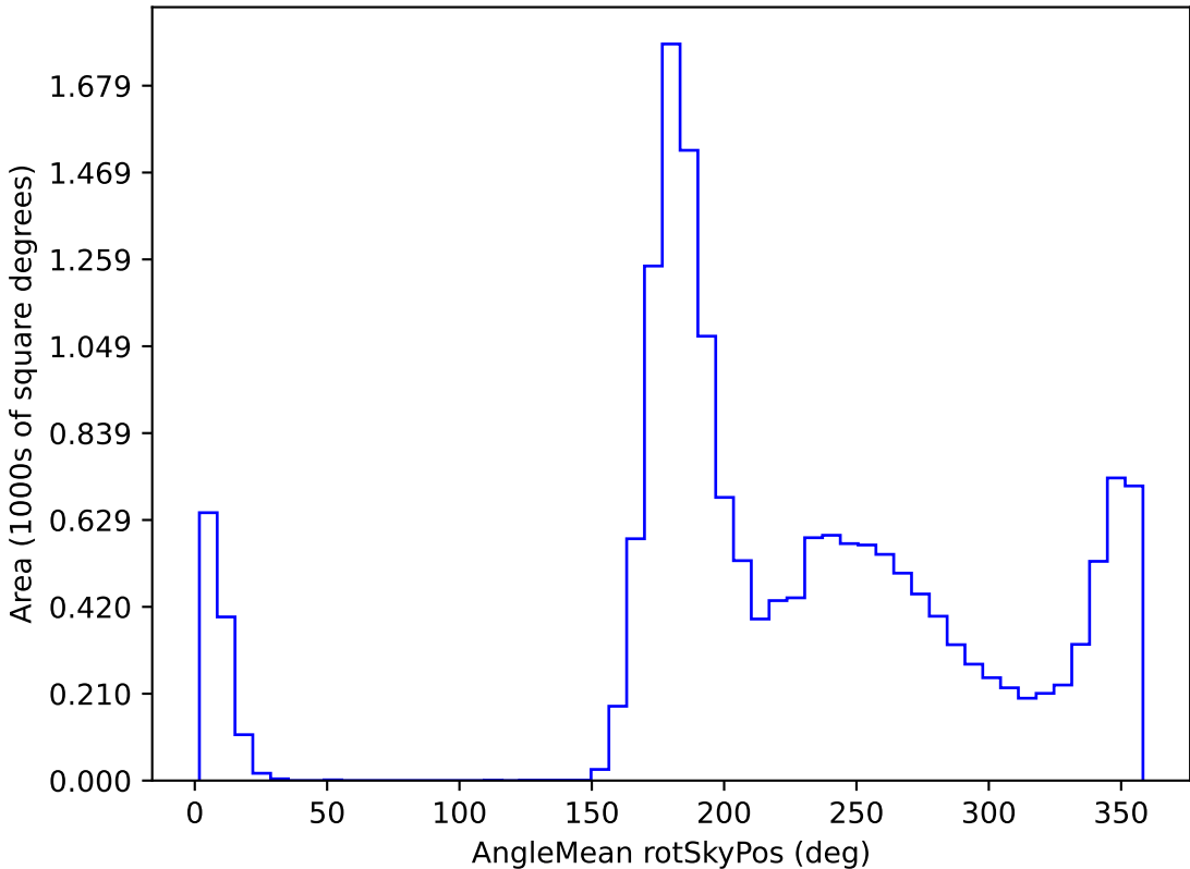
too_elab_r64_d2_gz_v3.4_10yrs WFD y band: AngleMean rotSkyPos
