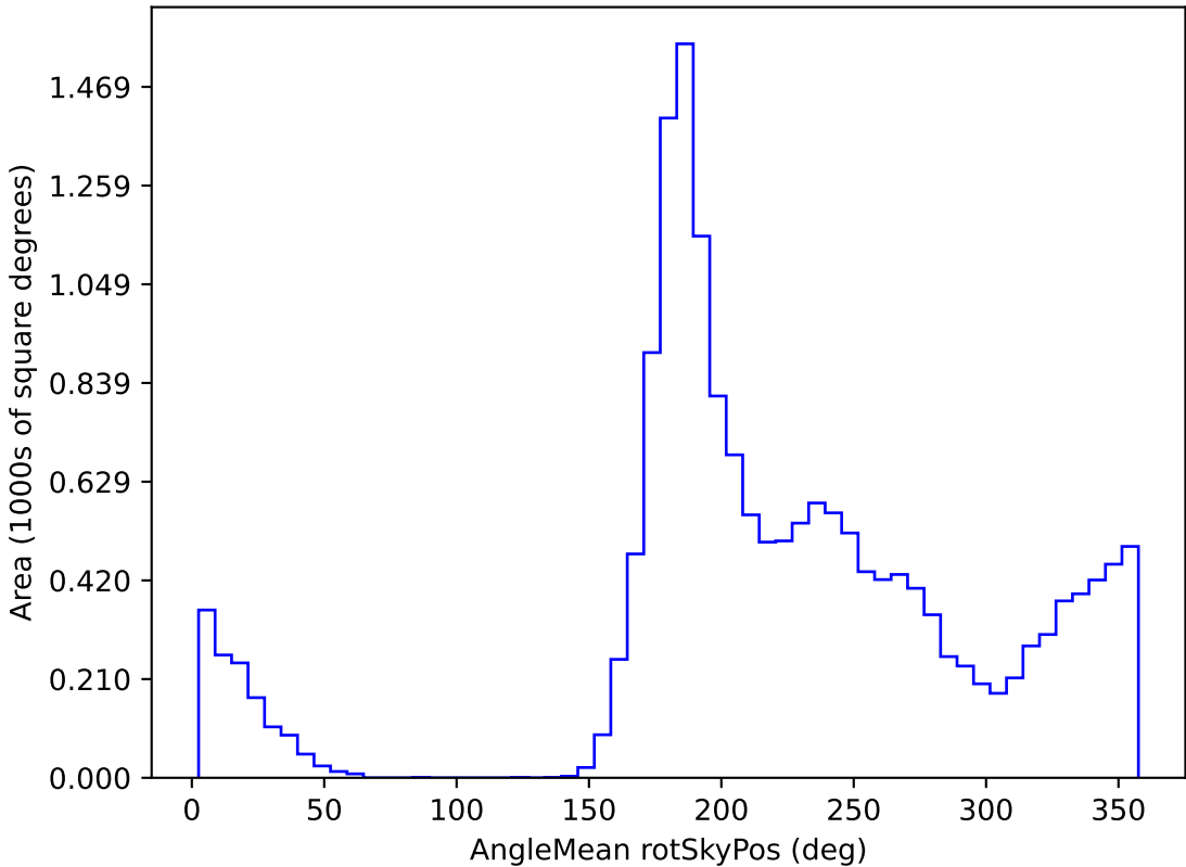
too_elab_r64_d2_gz_v3.4_10yrs WFD u band: AngleMean rotSkyPos
