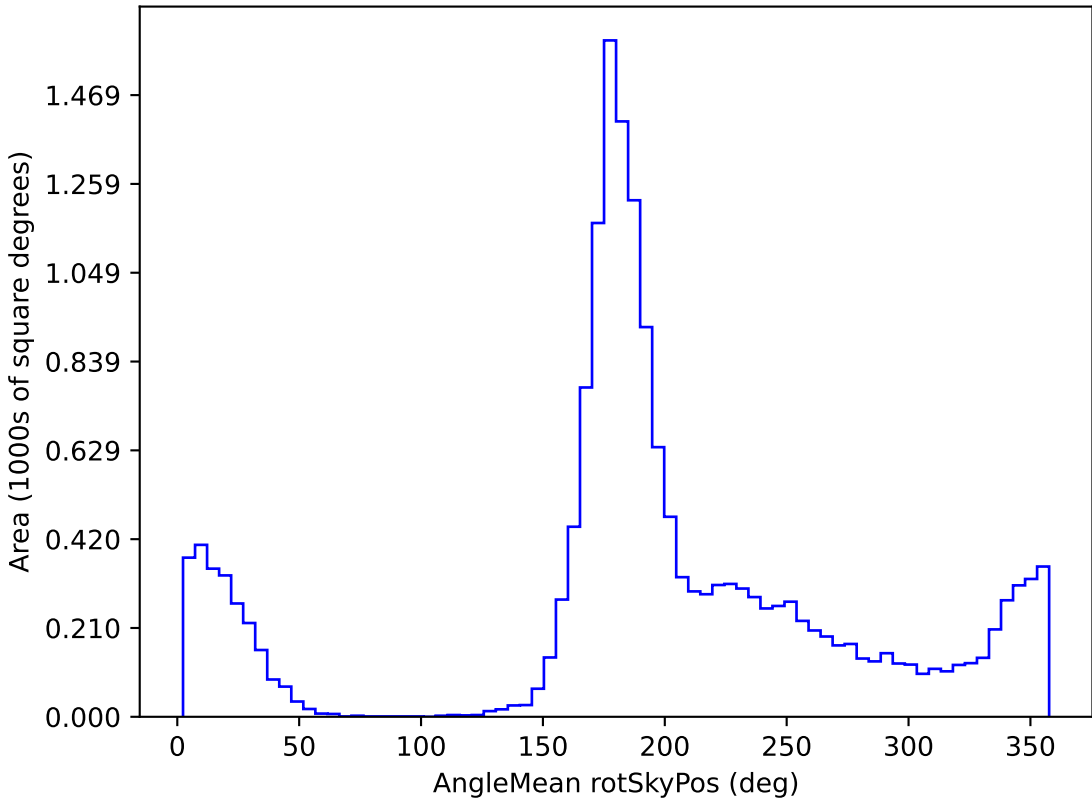
too_elab_r64_d2_gz_v3.4_10yrs WFD g band: AngleMean rotSkyPos
