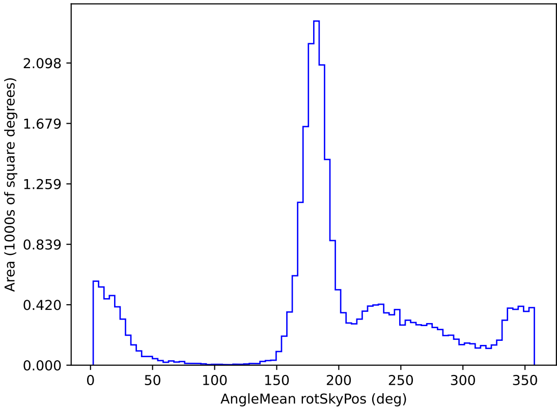
too_elab_r64_d2_gz_v3.4_10yrs All sky r band: AngleMean rotSkyPos
