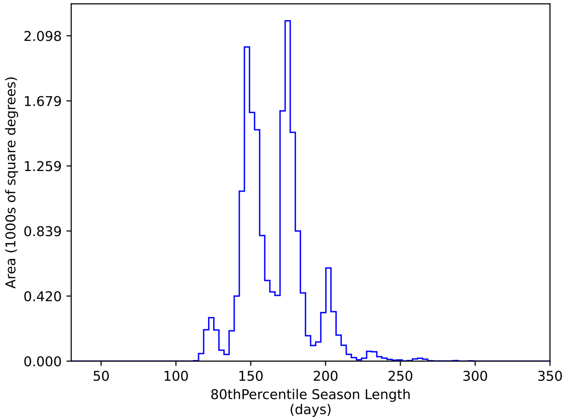
too_elab_r64_d2_gz_v3.4_10yrs WFD y band: 80thPercentile Season Length
