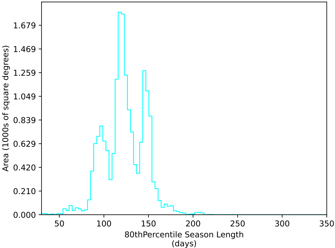
too_elab_r64_d2_gz_v3.4_10yrs WFD u band: 80thPercentile Season Length
