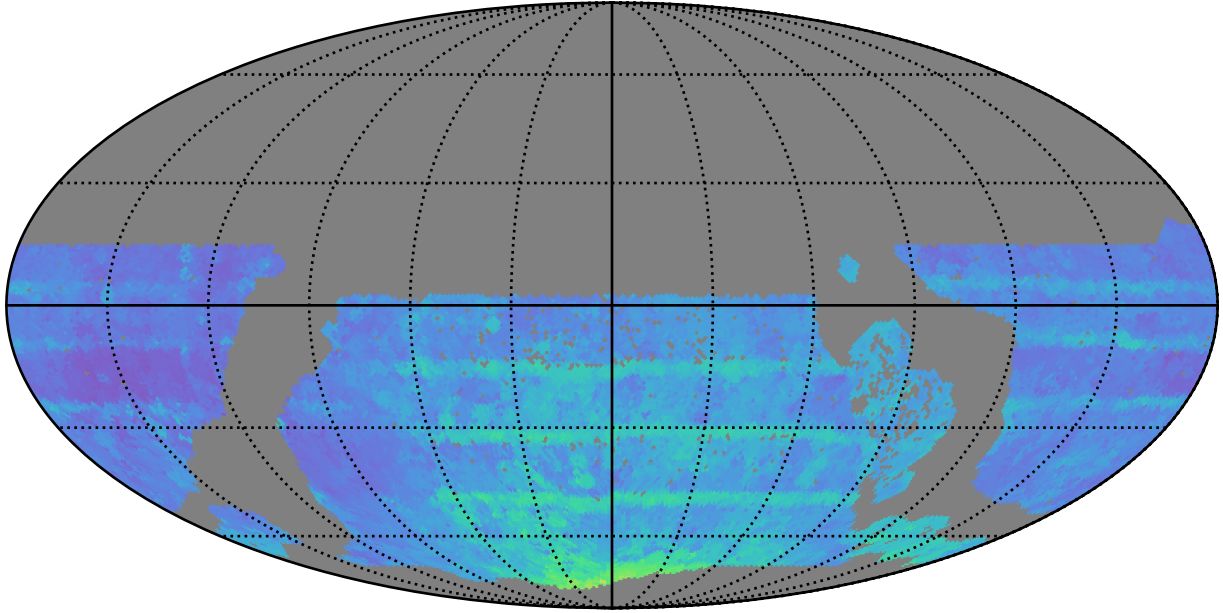
too_elab_r64_d2_gz_v3.4_10yrs WFD all bands: 80thPercentile Season Length
