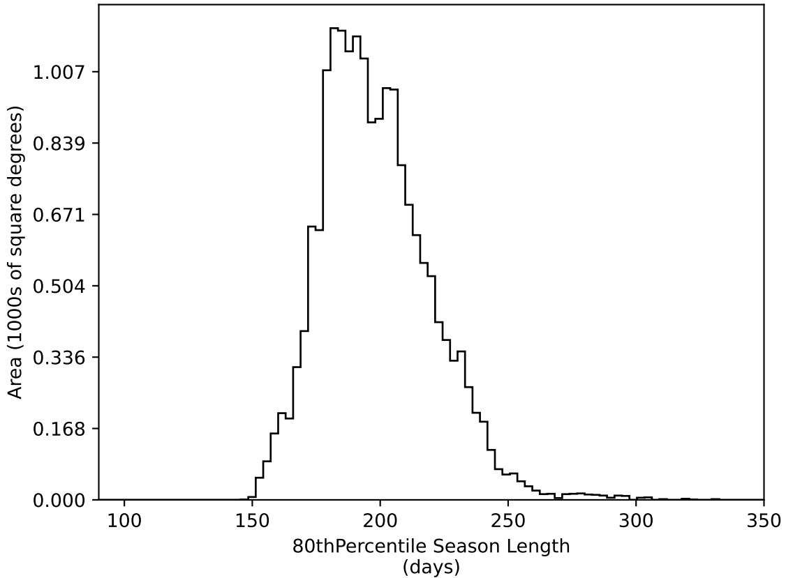
too_elab_r64_d2_gz_v3.4_10yrs WFD all bands: 80thPercentile Season Length
