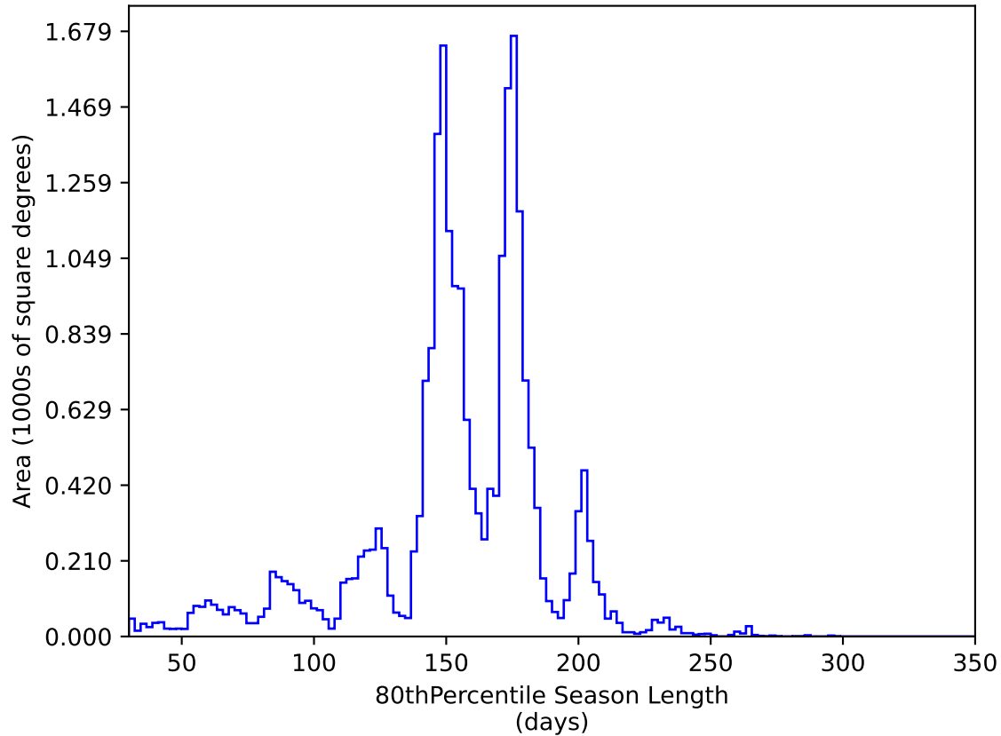
too_elab_r64_d2_gz_v3.4_10yrs All sky y band: 80thPercentile Season Length
