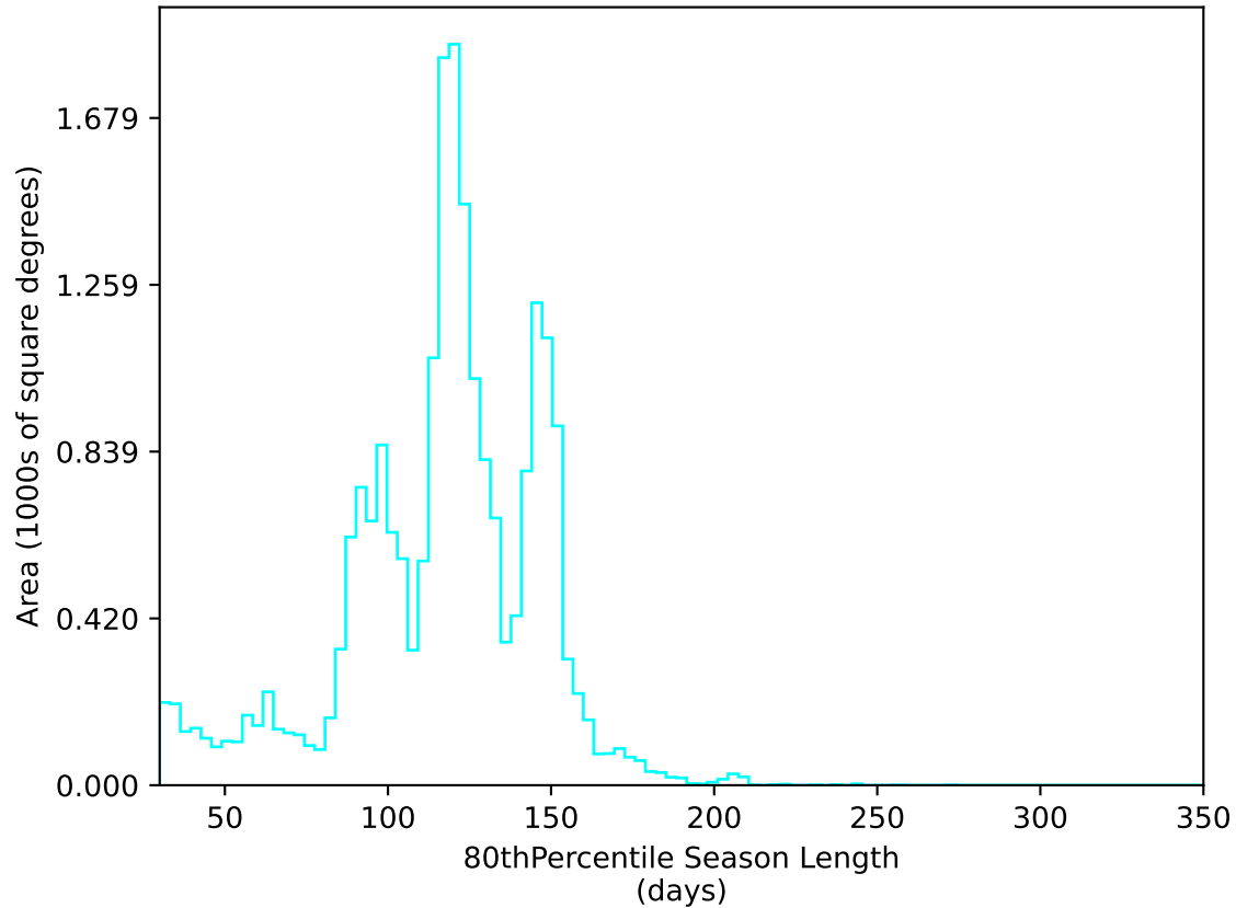
too_elab_r64_d2_gz_v3.4_10yrs All sky u band: 80thPercentile Season Length
