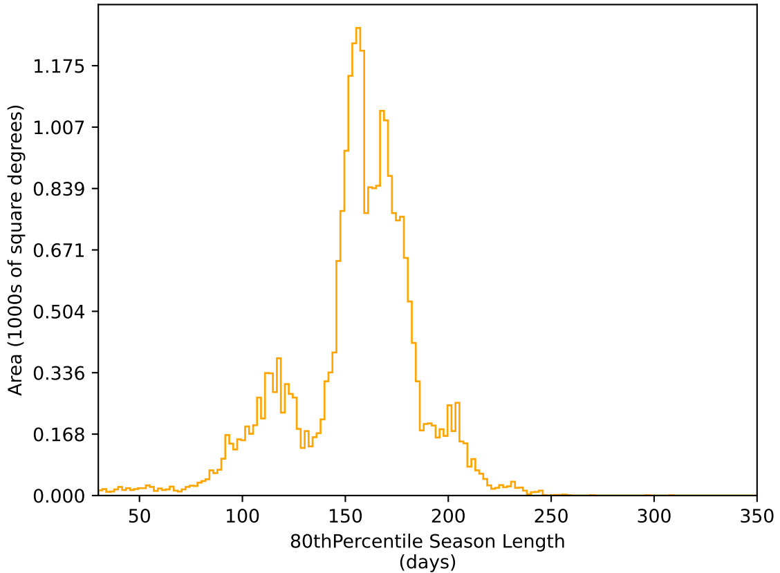
too_elab_r64_d2_gz_v3.4_10yrs All sky r band: 80thPercentile Season Length
