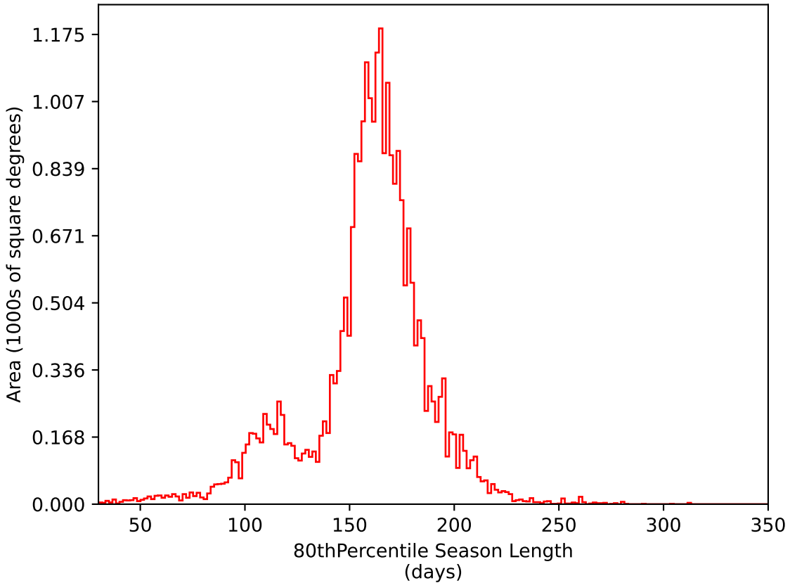
too_elab_r64_d2_gz_v3.4_10yrs All sky i band: 80thPercentile Season Length
