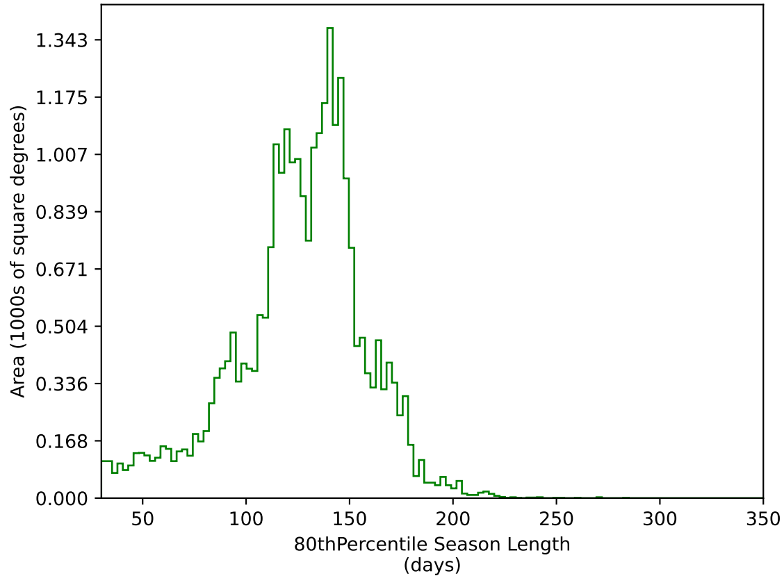
too_elab_r64_d2_gz_v3.4_10yrs All sky g band: 80thPercentile Season Length
