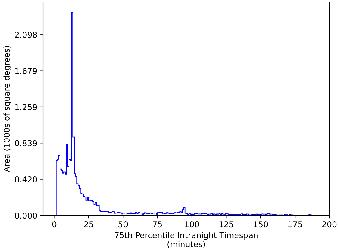
too_elab_r64_d2_gz_v3.4_10yrs WFD z band: 75th Percentile Intranight Timespan
