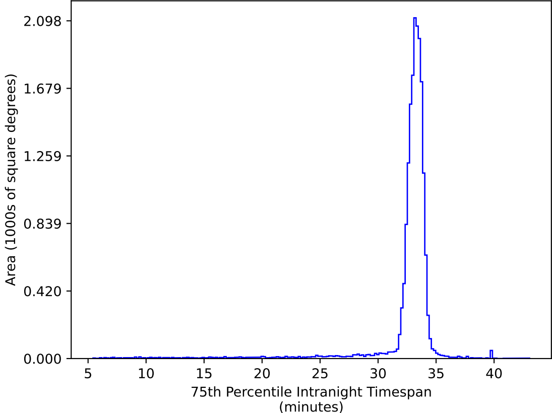
too_elab_r64_d2_gz_v3.4_10yrs WFD ug bands: 75th Percentile Intranight Timespan
